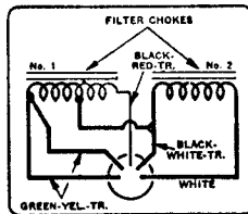
FILTER-CHOKES ASSEMBLY
